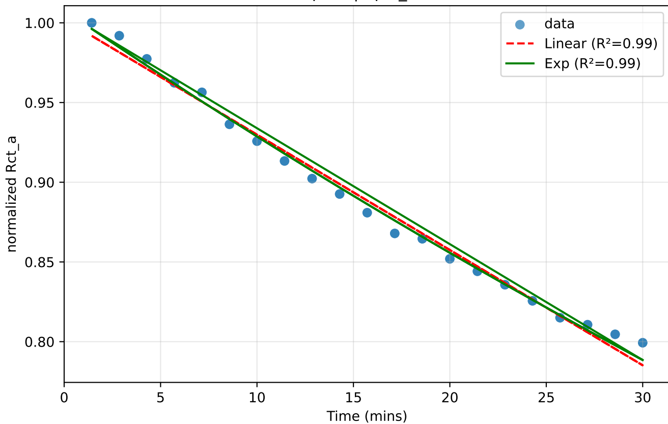
Chip 40 | 0pM_disso
